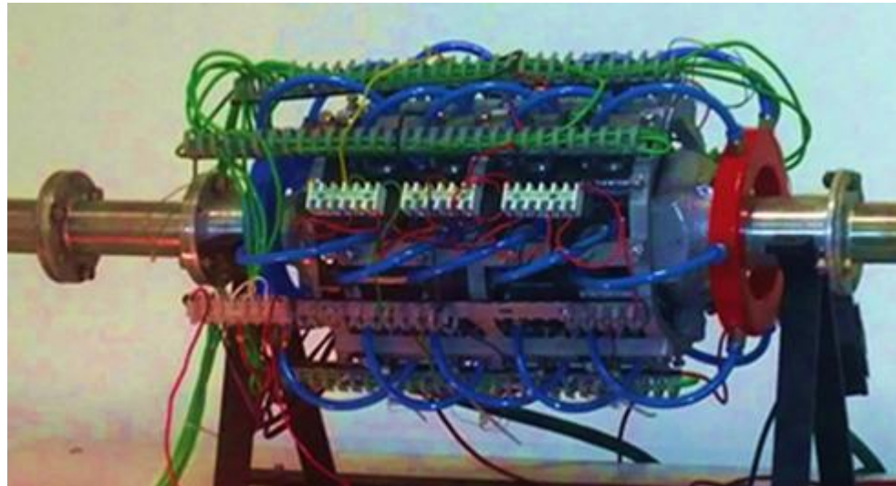
prototype of TEG (200 W)
