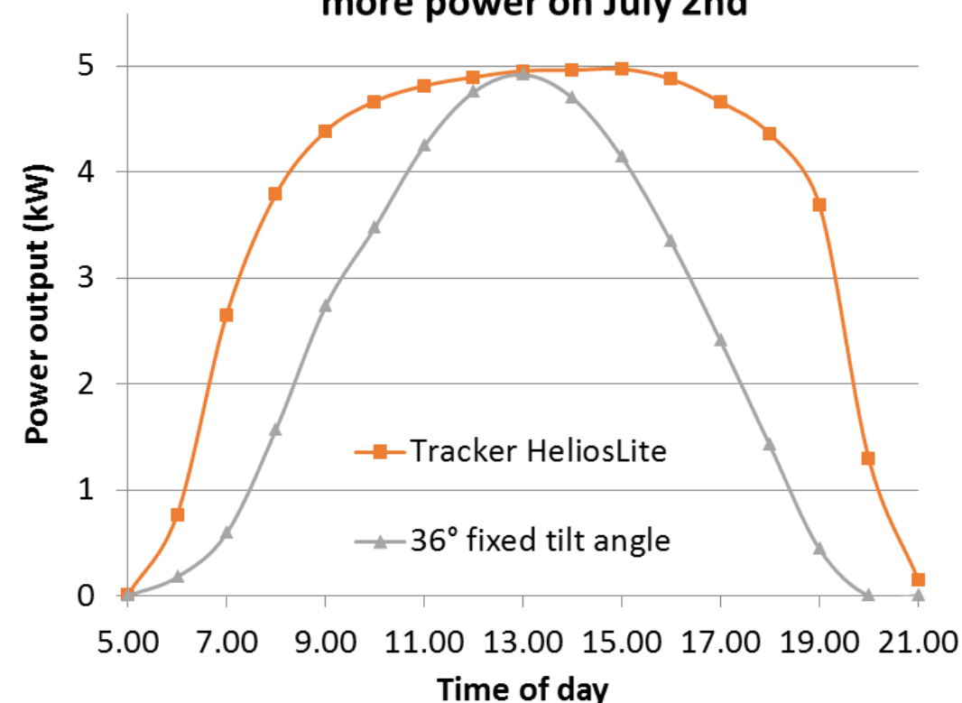
HeliosLite tracker at Solar Decathlon : 50% more power on July 2nd
